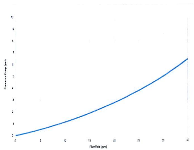
3/4" Short Headloss Curve
